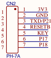
Indicator Port Key And Reset Key Interface
