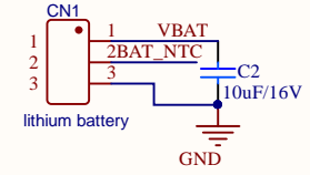
Lithium Battery Interface
