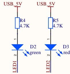
Charging Indicator
