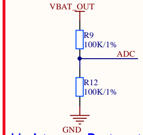
Voltage Detection
