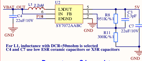
Booster Circuit
