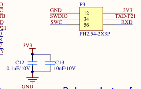
Debug Interface
