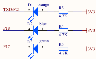
Indicator Light
