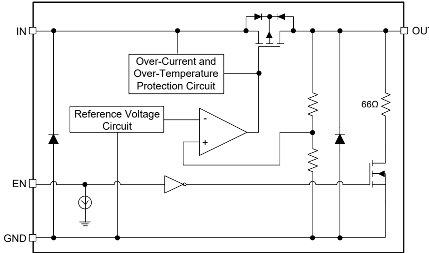
Figure 1. Block Diagram
