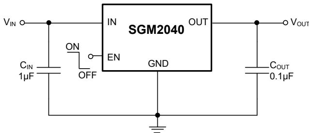
Figure 2. Standard Circuit
