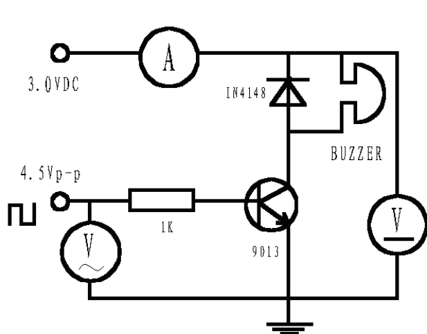
Test Circuit
