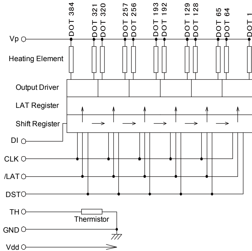
Figure 3-6 Thermal Head Block Diagram
