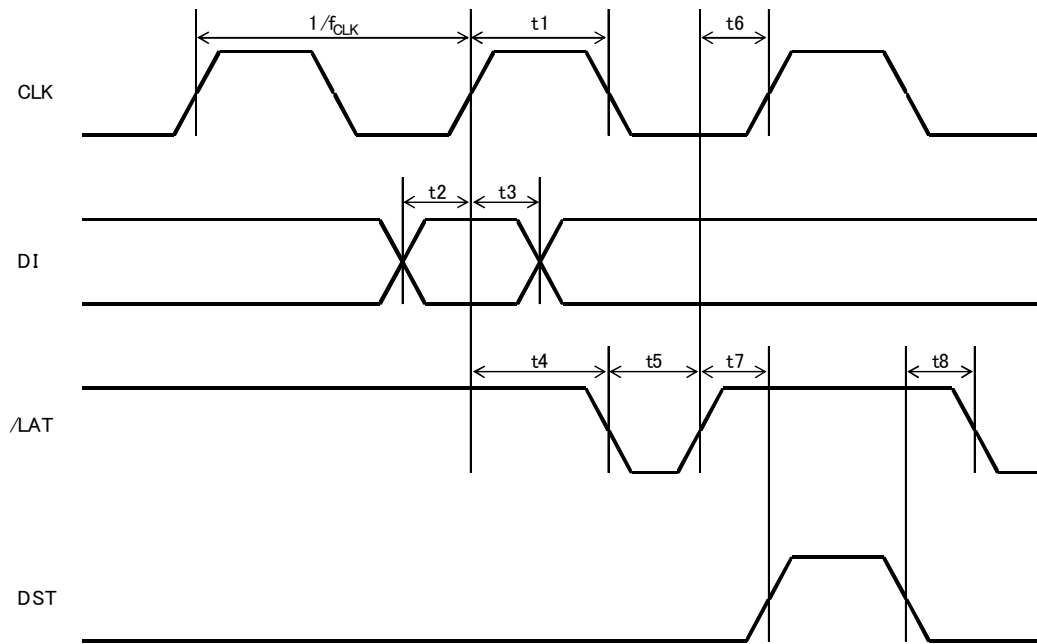
Figure 3-8 Thermal Head Drive Timing Chart
