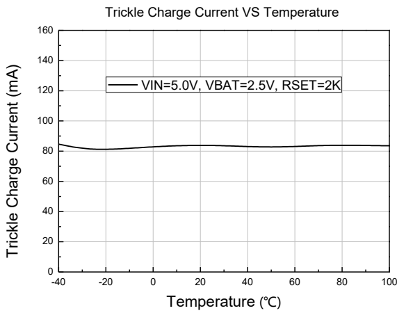
17. Charge Current VS Temperature
