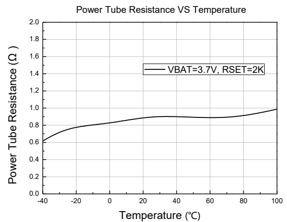
18. Power Tube Resistance VS Temperature
