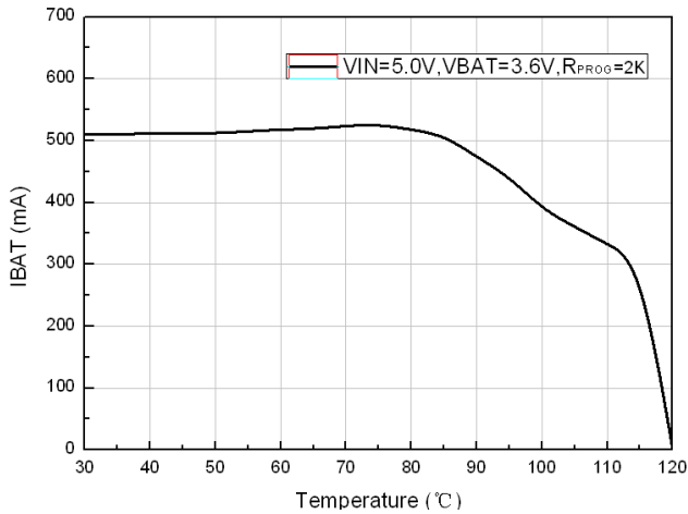
17. Charge Current VS Temperature
