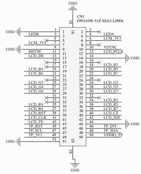
T35P1280Q-02 LCD RGB Interface RGB Interface LCD Connector
