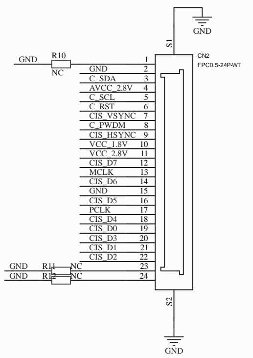
OVX4388 CMOS Camera Module Interface DVP Interface Connector
