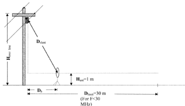
Figure 1 – Illustration of Slant-Range Distance
